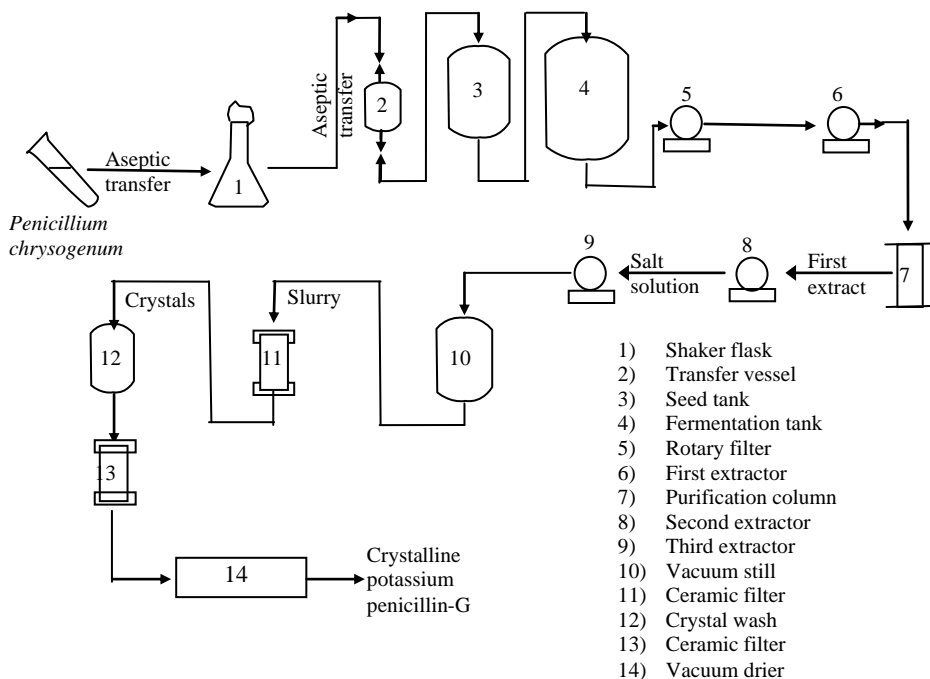
Figure 9.6: Flow Sheet for Large-Scale Production of Penicillin
