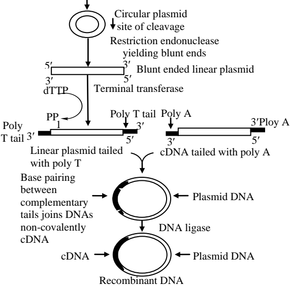
Figure 3.7: Homopolymer Tailing
