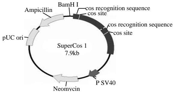
Figure 3.12: Cosmid
