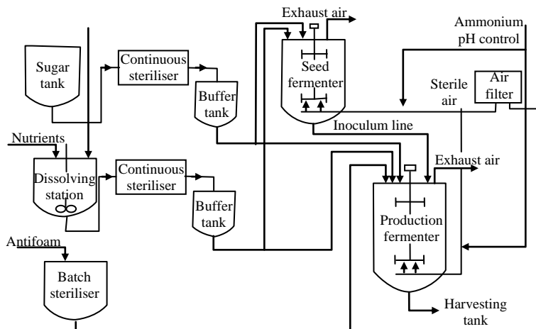
Figure 9.11: Flow Diagram of Commercial Production Method of Glutamic Acid (Glutamate)
