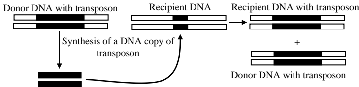
Figure 7.11: Replicative Transposons
