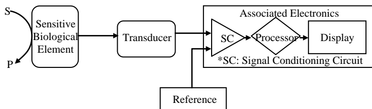
Figure 2.1: Schematic Diagram Showing Main Components of a Biosensor
