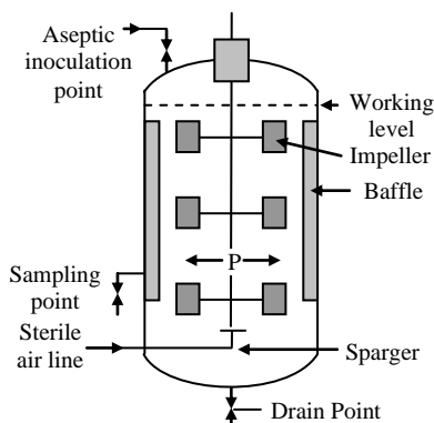
Figure 9.3: Diagram of a Typical Fermenter
