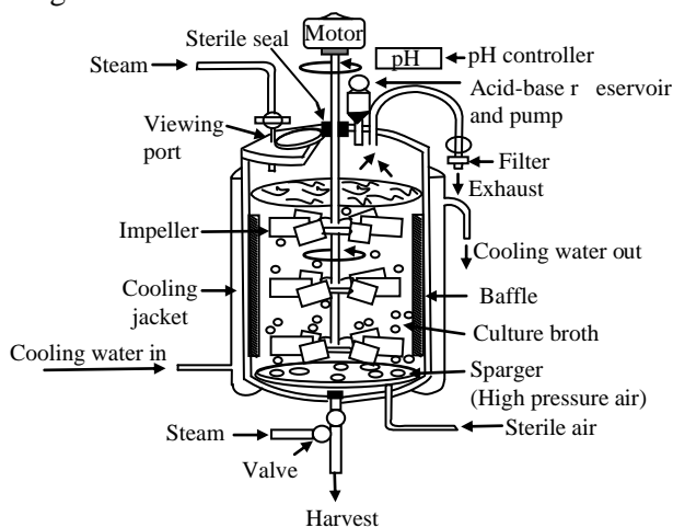
Figure 9.4: Internal View of an Industrial Aerobic Fermenter
